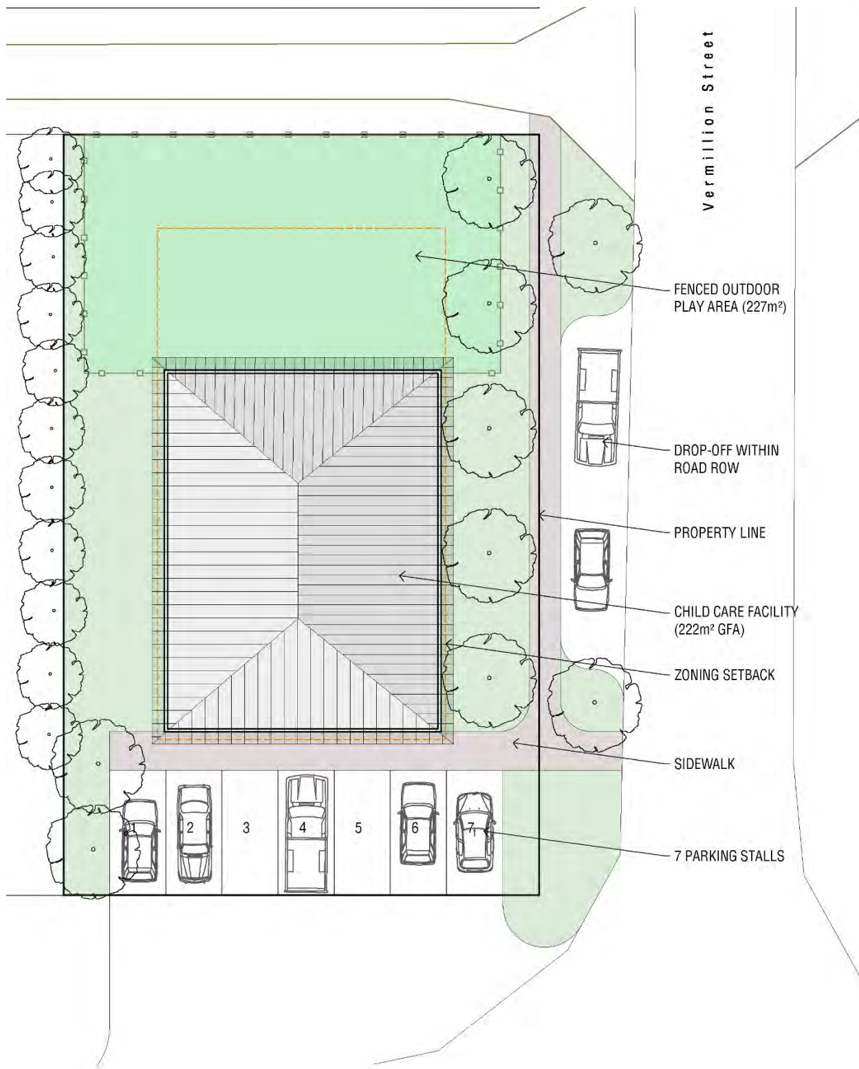
Figure 11 – Vermillion Property – Site Plan, Option 1
