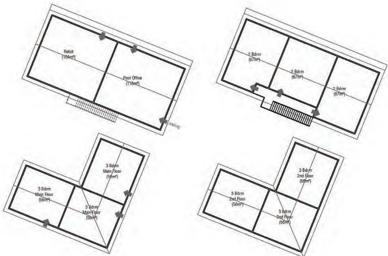
Conceptual Floor Plans - Main Floor Plan (left) and Upper Floor Plans (right)
