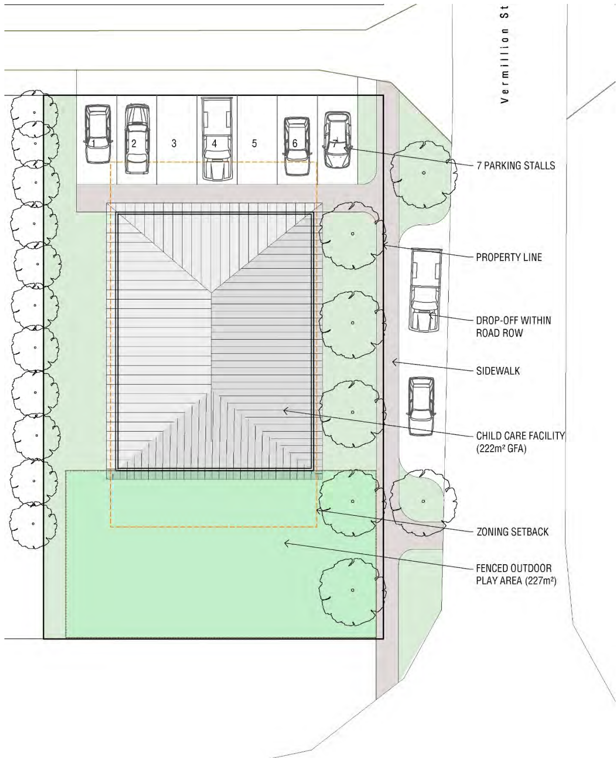
Figure 12 – Vermillion Property – Site Plan, Option 2
