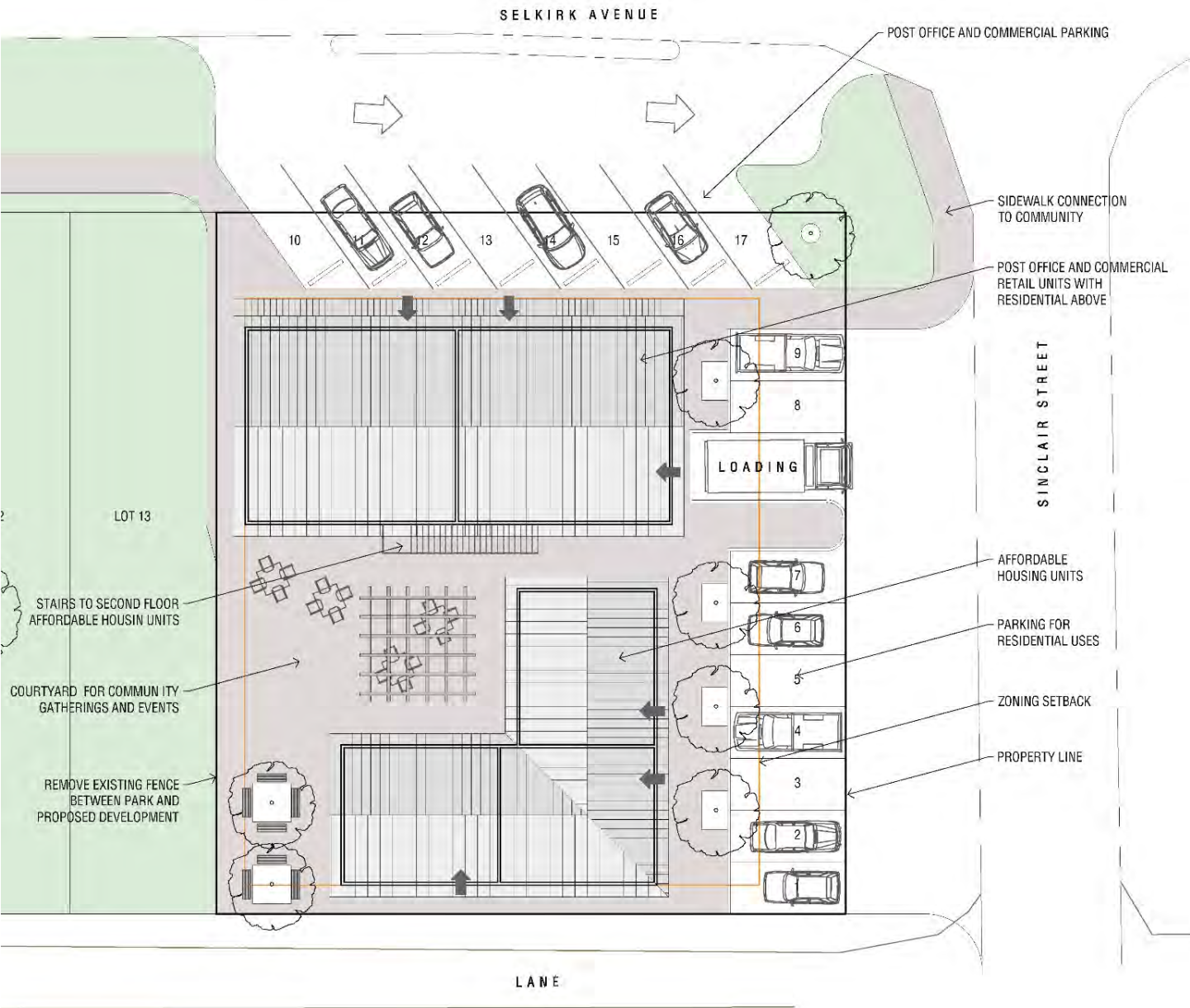
Figure13 – Post Office Property – Site Plan
