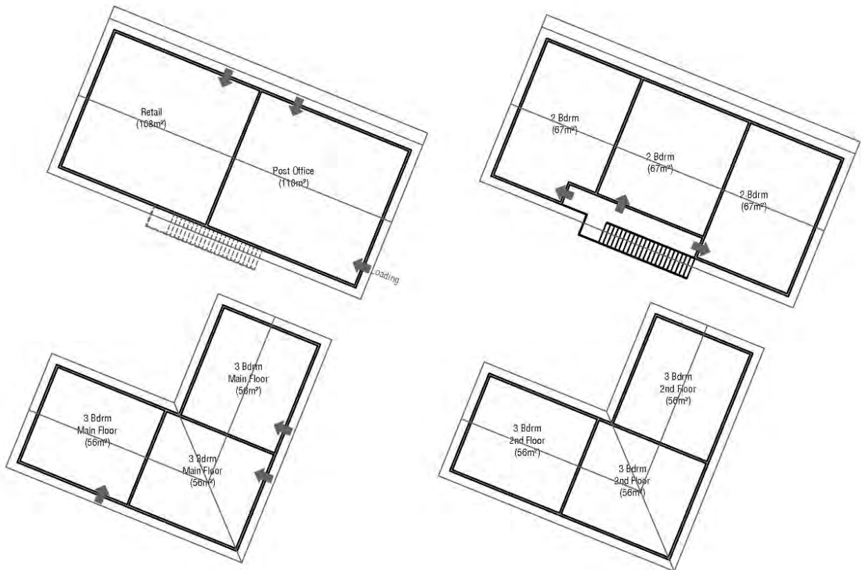
Figure 10 – Conceptual Floorplans – Main Floor Plan (above left) and Upper Floor Plan (above, right)
