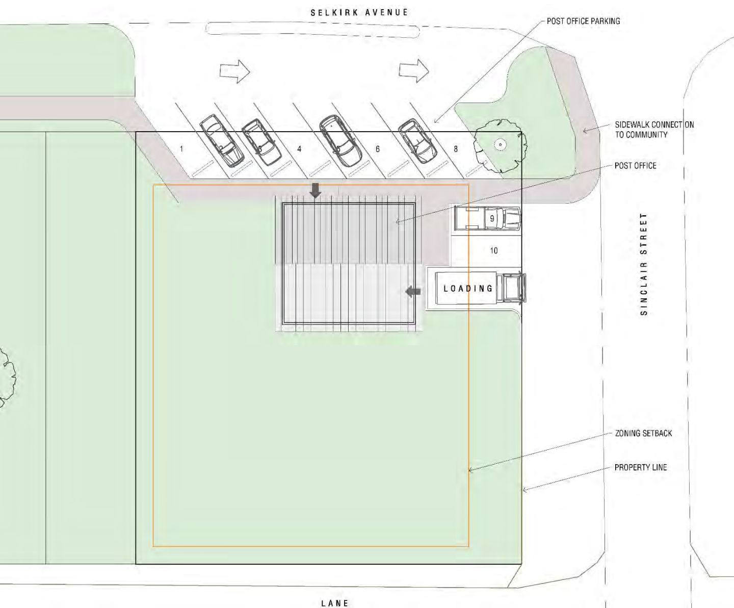
Figure 15 – Post Office Property, Site Plan, Phase 1
